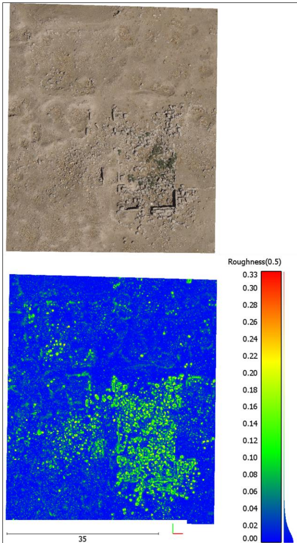
Figure 13. Surface roughness analysis of Small Mosque.
