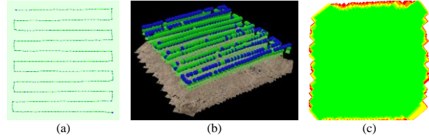
Figure 4. Adjusted coordinates of aerial photographs (a), point cloud (b) and image overlays of the land surface (c).
